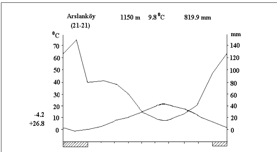
Fig. 2. Ombrothermic diagram of Arslanköy.
