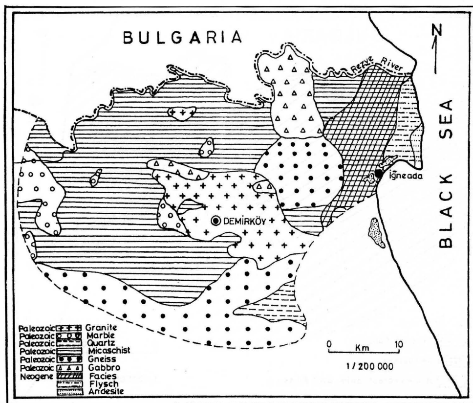
Fig. 5. Geological map of the study area.
