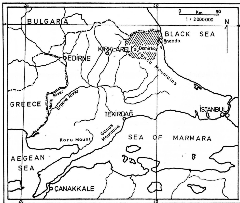
Fig. 1. The study area in European Turkey.
