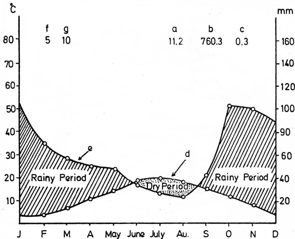
Fig. 3. The climatological diagram of Demirköy station (in the centre of the study area). a, average annual temperature (°C); b, average annual rain (mm); c, minimum average warmth of the coldest month (°C); d, temperature graph; e, rain graph; f, temperature measuring years number; g, rain measuring years number.
