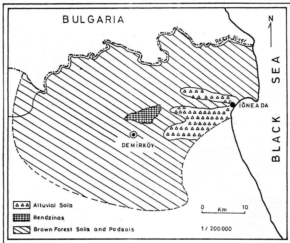
Fig. 4. Soil map in the study area.
